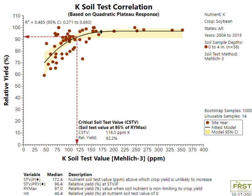
Figure 1. Example correlation between soybean relative yield and Mehlich-3 K using quadratic plateau model with the critical soil test value (CSTV) interpreted at 95% of the plateau yield.
